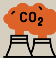
Increased Green House Gases
