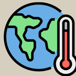
Accelerated Climate Change
